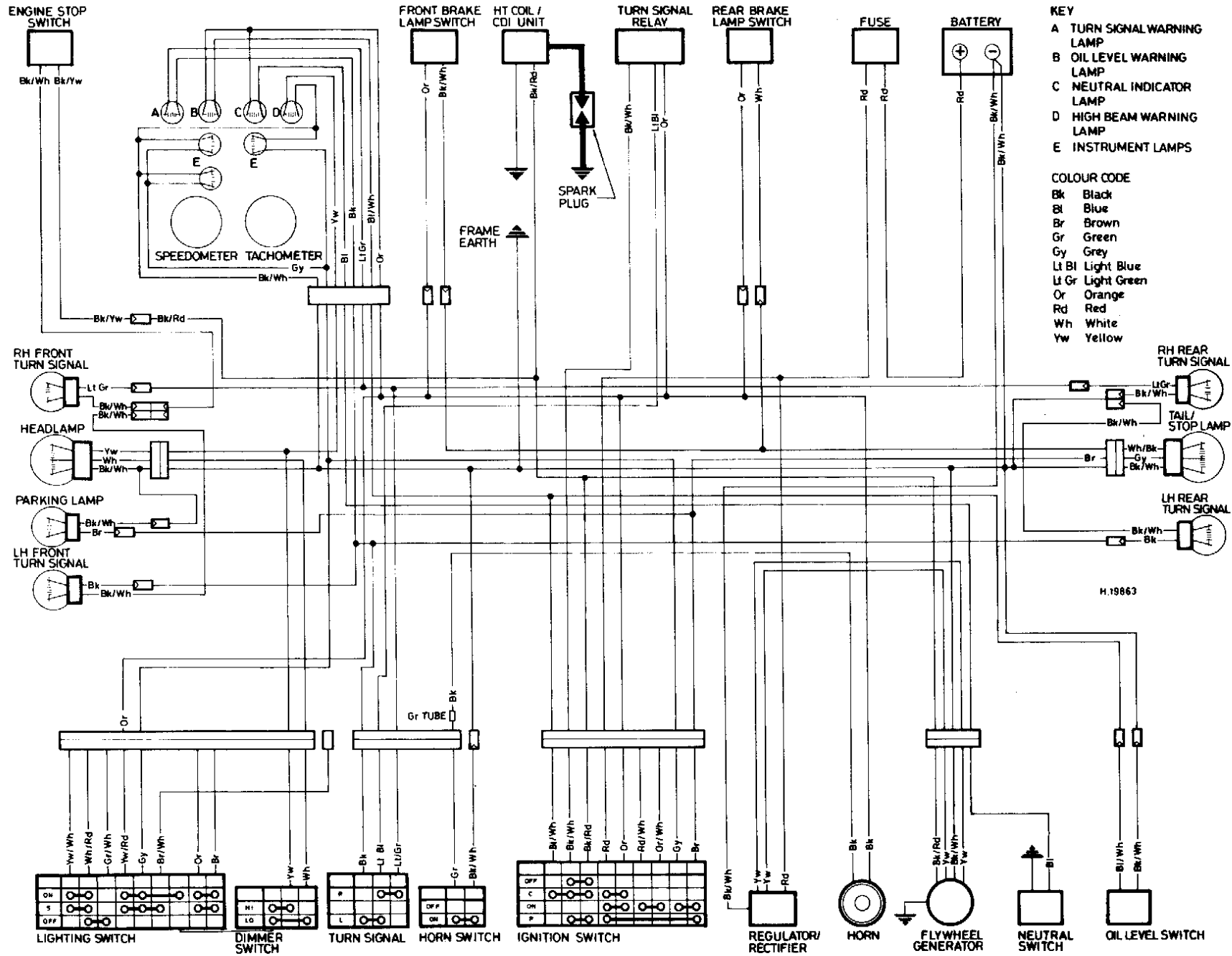
Wiring diagram
